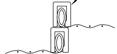
6 JAMB DETAIL SCALE: FULL
