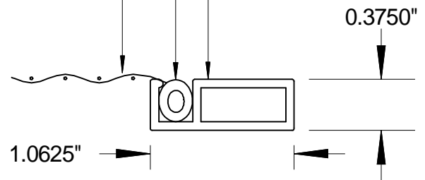
1 JAMB DETAIL SCALE: FULL HEAD and SILL SIMILAR
